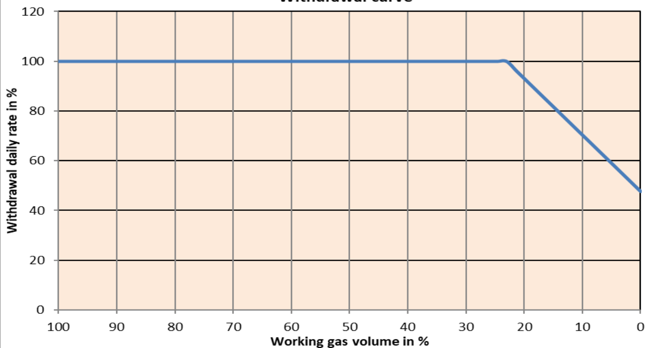
Withdrawal curve
