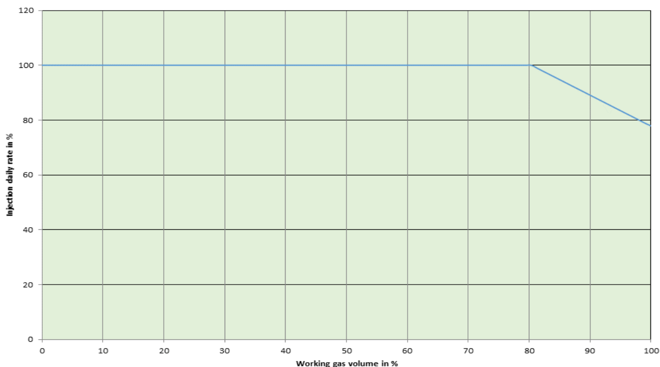
Injection curve
